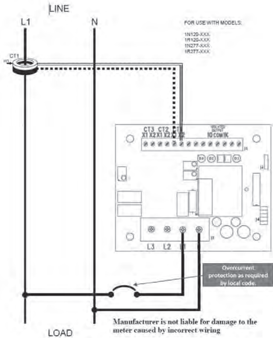
Figure 7: 1-phase, 2-wire Hookup Diagram
