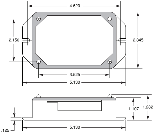
Figure 1 - Mini Meter Dimensions, in inches
