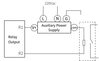
Relay output
