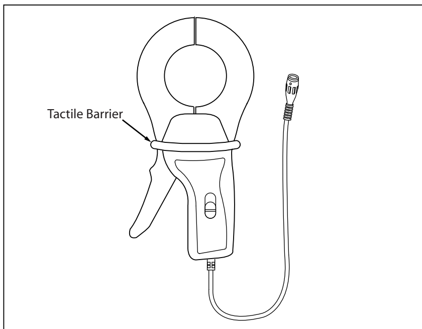
Figure 1. i1000s AC Current Probe
