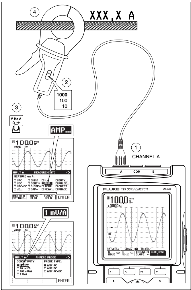
Figure 3. ScopeMeter Setups
