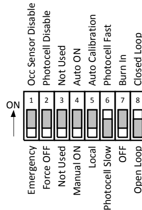
DIP SWITCH BANK S2
