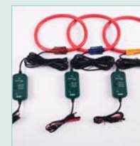
Model PQ34-30 3000A (24"/600mm) Flexible Current Clamp Probes for wrapping around busbars
