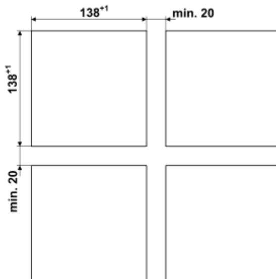
Panel cutout PQ3K
